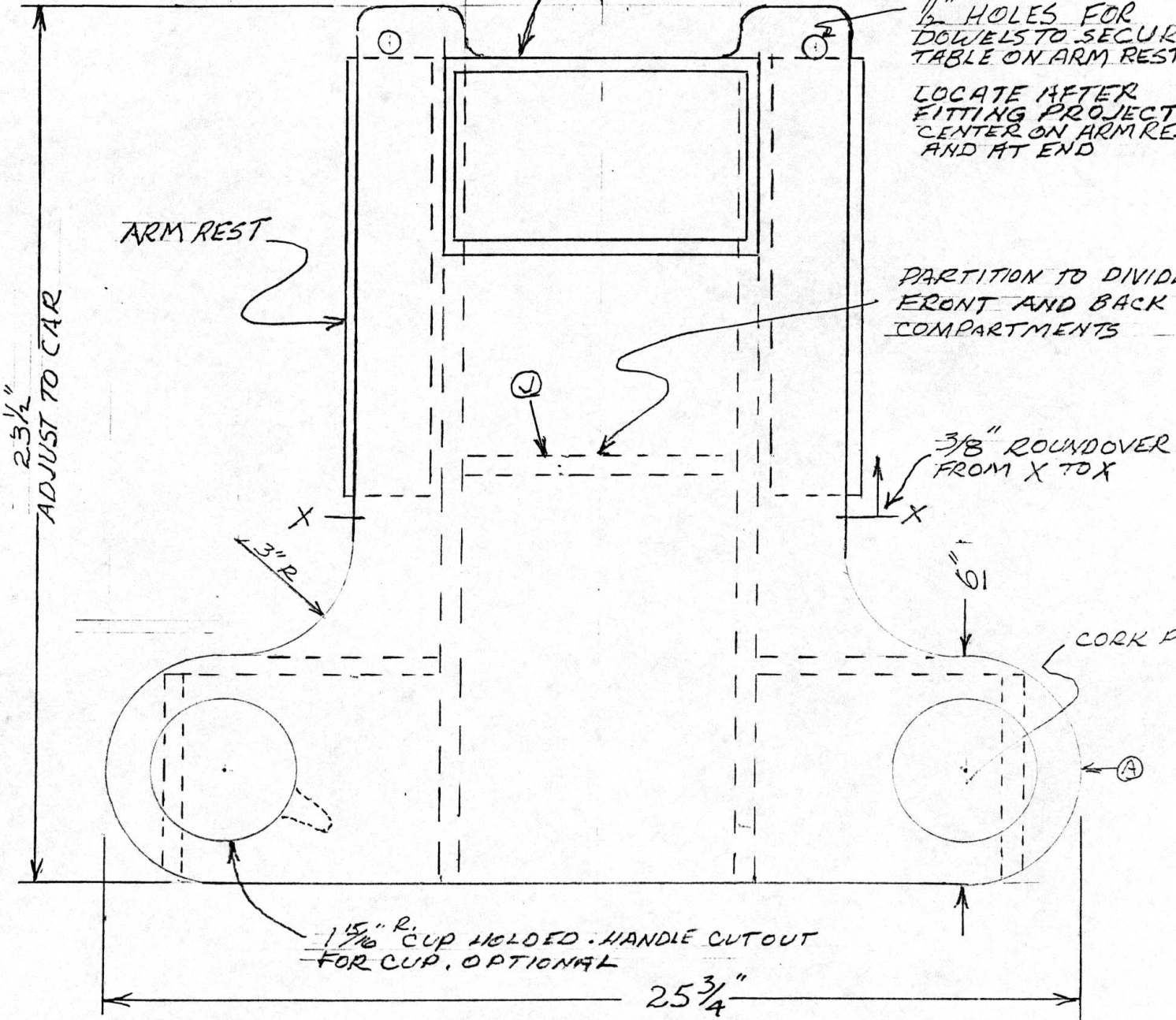
TOP VIEW
